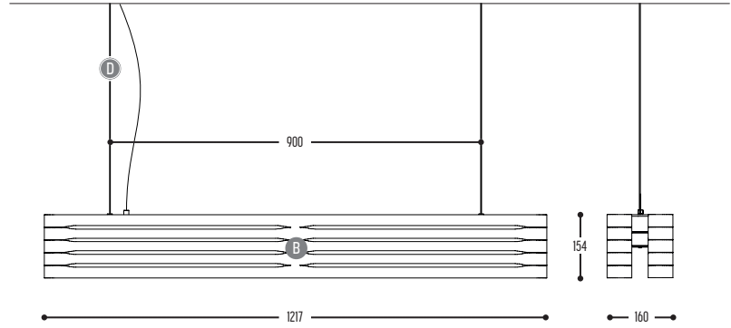
ORGUE 1363-BB(B)-866003-DD-K
