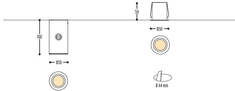
TAQI BOX 1 2700-BB-906603-K
