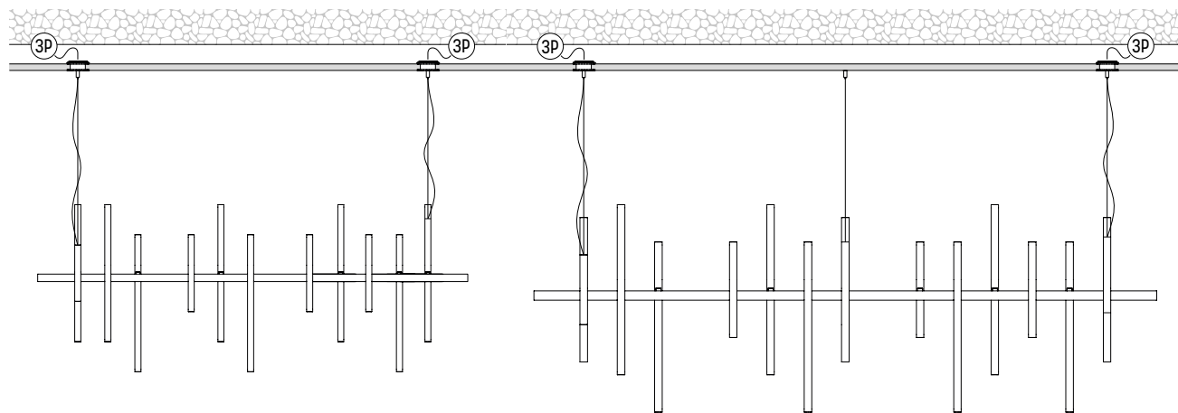
EQUALIZER 1600 / 08 NON-DIM or DALI/PUSH-DIM 3501-BB(B)-903H-DD-K-2-08
